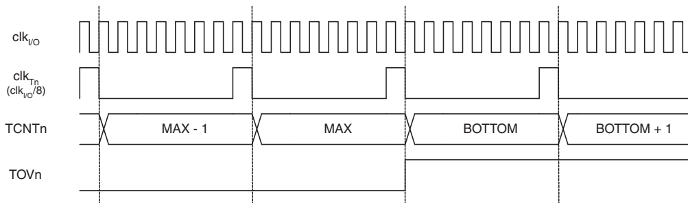
Figure 15-9. Timer/Counter Timing Diagram, with Prescaler ( f_{\text{clk}_{I/O}}/8 )
