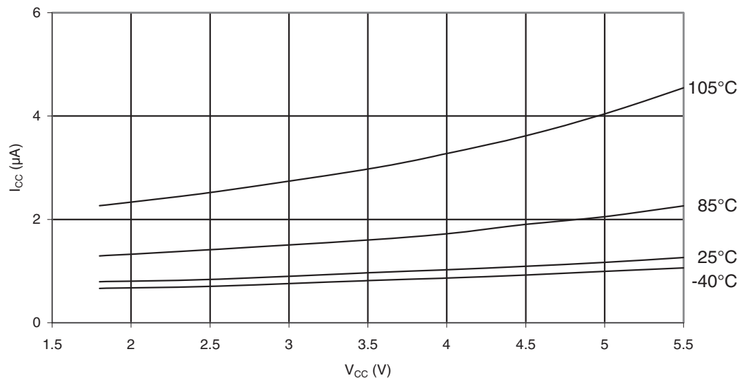
Figure 33-13. ATmega88PA: Power-Save Supply Current vs. V_{CC} (Watchdog Timer Disabled and 32kHz Crystal Oscillator Running)
