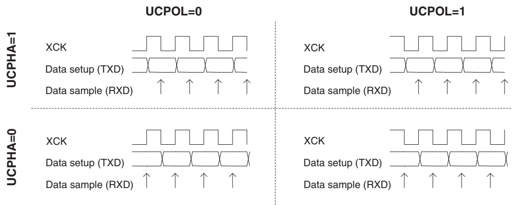
Figure 21-1. UCPHA n and UCPL n data transfer timing diagrams.
