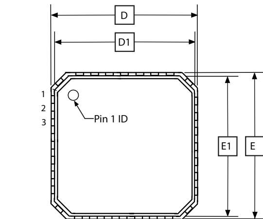
TOP VIEW W
