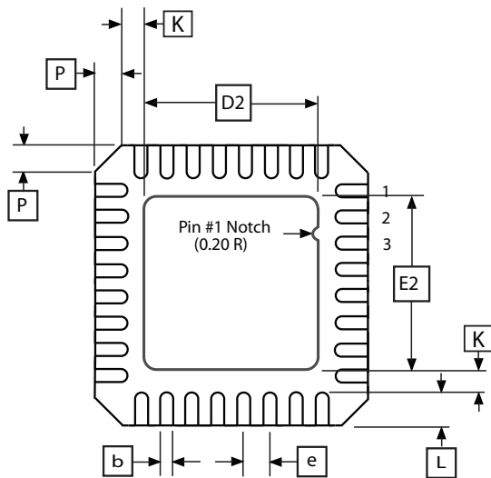
BOTTOM VIEW W
