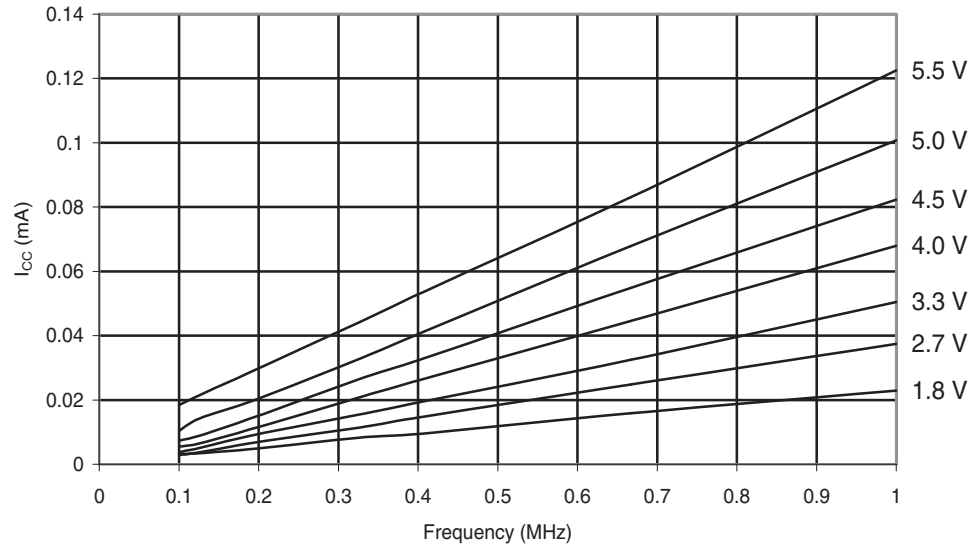
Figure 31-45. ATmega48A: Reset Supply Current vs. Low Frequency (0.1 - 1.0MHz)
